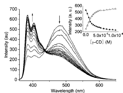
Figure 3. Change of fluorescence spectra of 2c with \gamma -CD in water. \lambda_{\text{ex}} = 330 nm, ex/em slits = 5/5 nm. [\mathbf{2c}] = 5.0 \times 10^{-5} M. Inset, curves of fluorescence intensity vs concentration of \gamma -CD measured at 485 nm (▲) and 405 nm (Δ).
