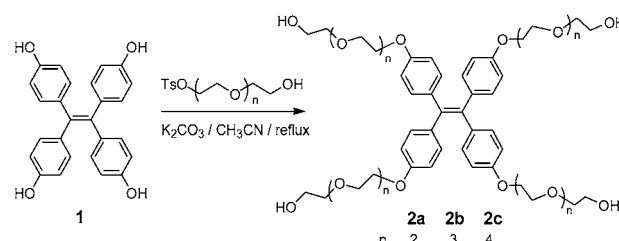
Figure 1. Synthesis of the AIE compounds 2a–2c .
