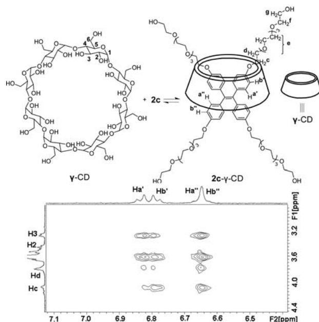
Figure 5. Schematic structure of 2c - \gamma -CD inclusion complex and its partial 2D NOESY spectrum in \text{D}_2\text{O} . [\text{2c}] = [\gamma\text{-CD}] = 2 \text{ mM} .
