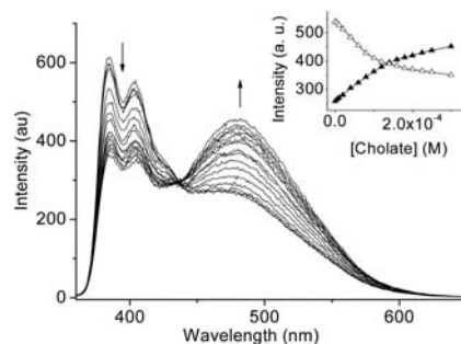
Figure 6. Change of fluorescence spectra of 2c - \gamma -CD complex with the cholate in water. \lambda_{\text{ex}} = 330 \text{ nm} , ex/em slits = 5/5 nm. [\text{2c}] = [\gamma\text{-CD}] = 5.0 \times 10^{-5} \text{ M} . Inset, curves of intensity vs the cholate concentration measured at 485 nm ( \blacktriangle ) and 405 nm ( \triangle ).
