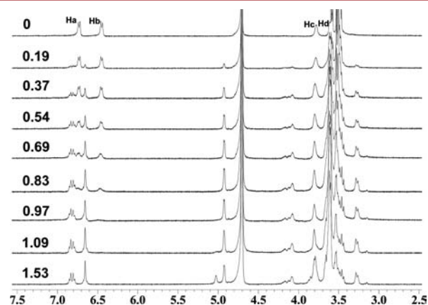
Figure 4. Change of 1 H NMR spectra of 2c with \gamma -CD in D 2 O. [\mathbf{2c}] = 2.0 mM. The number over the spectrum is the molar ratio of \gamma -CD vs 2c .
