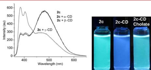
Figure 2. Fluorescence spectra of 2c without and with \alpha -CD, \beta -CD, and \gamma -CD in water. (Right) Photos of a solution of 2c , 2c - \gamma -CD, and 2c - \gamma -CD-potassium ursodeoxycholate in water under a 365 nm lamp. [\mathbf{2c}] = [\alpha\text{-CD}] = [\beta\text{-CD}] = [\gamma\text{-CD}] = 1/3[\text{cholate}] = 5.0 \times 10^{-5} M, \lambda_{\text{ex}} = 330 nm, ex/em slits = 5/5 nm.
